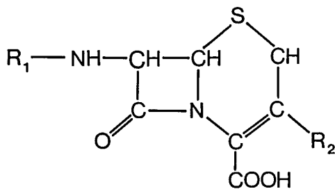
Figure 2. Basic structure of the cephalosporins.
