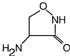
Figure 3. Structural formula of cycloserine.
